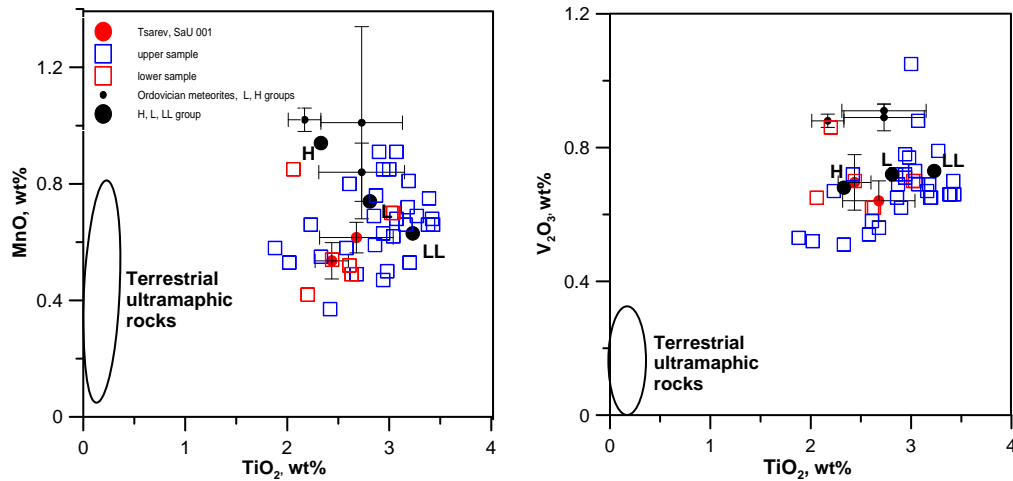
Fig. 1 a, b. Chemical compositions of chromite from the Ordovician rocks in Russia in comparison with chromite compositions of Tsarev and SaU 001 L5 chondrites, average chromite composition of Swedish Ordovician paleometeorites, and H, L, LL chondrites [7, 8].
