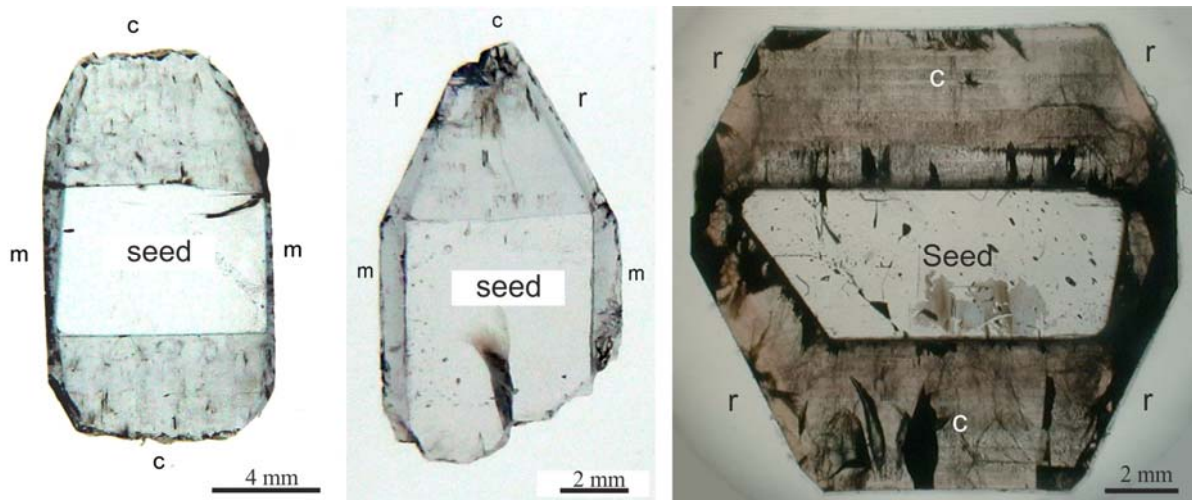
Figure 3. Internal sectorial-zone structure of synthetic Cr-containing topaz
