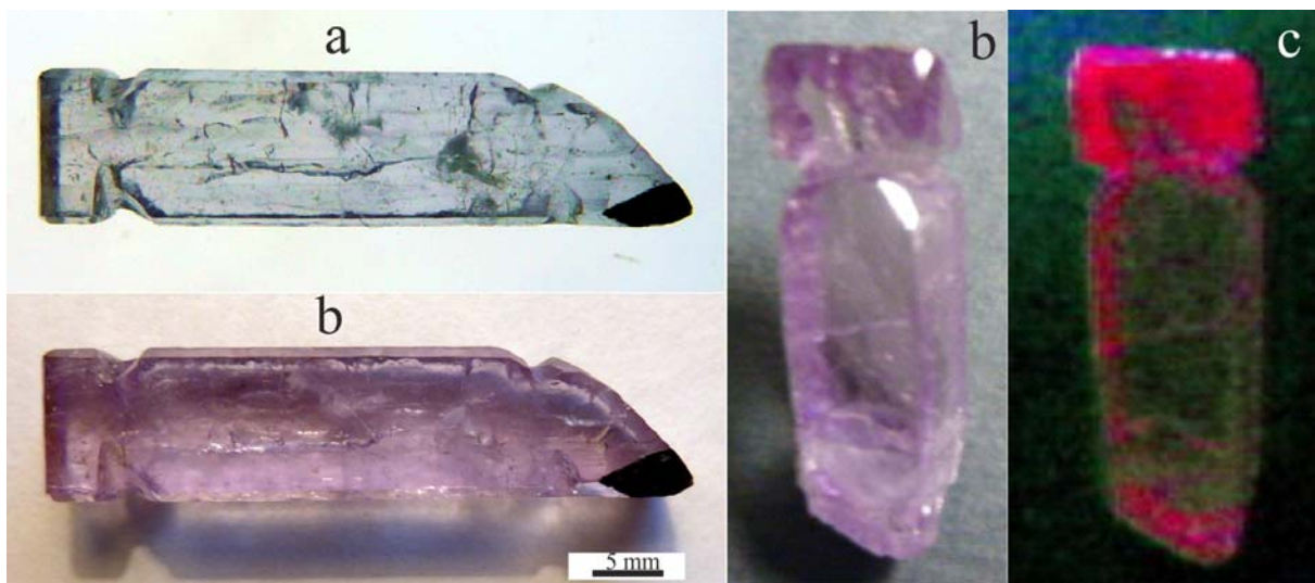
Figure 4. Colour of synthetic Cr-containing topaz at day (a), fluorescent lamp (b) and UV (c) illumination
